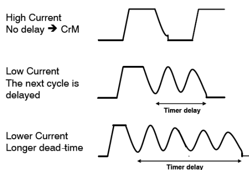
Figure 4. CCFF Operation
